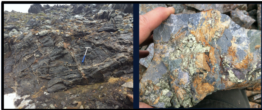
Figure 1. Example of stockwork vein zones flanking ridgeline outcrops at Burfjord.
